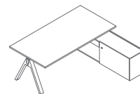
V04PM 2000 / 1800 / 740 120.22 kg
