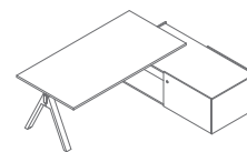
V06PM 2000 / 1000 / 740 154.22 kg
