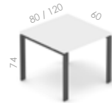
MWSK 0860 WU 80 / 60 / 74 [26]
