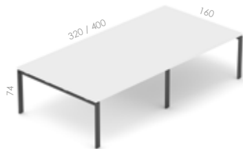
MWSK 32 U 320 / 160 / 74 [144]
