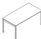
BOY04 1600 / 800 / 740 44.35 kg
