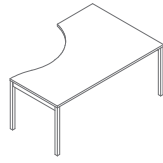
BOY17 1800 / 1200 / 740 51 kg
