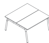
BOW44 1400 / 1410 / 740 61.2 kg
